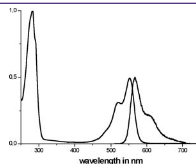
Spectrum of Chromeo™ 546 conjugated to Streptavidin.
